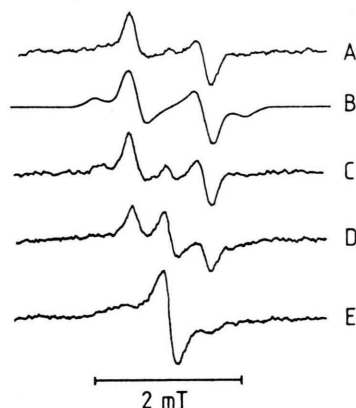
Fig. 1. Derivative wide-line H-NMR spectra of hydrated zeolites at 90 K. A: Linde 13X (Na-X) with 3.5 H_2O /cage (37 mg H_2O /g), only in the supercages. B: Calculated derivative doublet powder spectrum with Gauß broadening. C: Linde 13X with 3.5 H_2O /cage in sorption equilibrium. D: Linde 13X with 5.4 H_2O /cage after washing with 2.5 L H_2O /g at 295 K in 3 days. E: (Na, H)-ZK-5 with 3.5 H_2O /cage.
